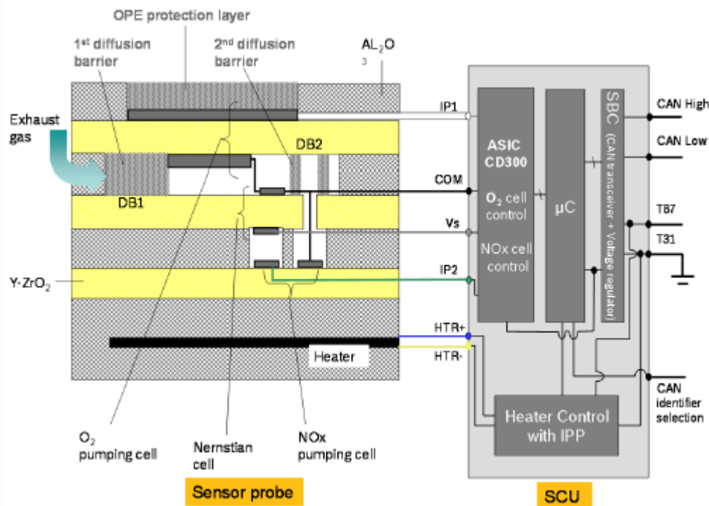
Figure 3: NOx Sensor operation diagram
