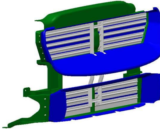
Figure above: This figure shows a grill shutter viewed from the outside grill for 3.0L only. The blue parts form a duct keeping incoming air from flowing around the radiator.
